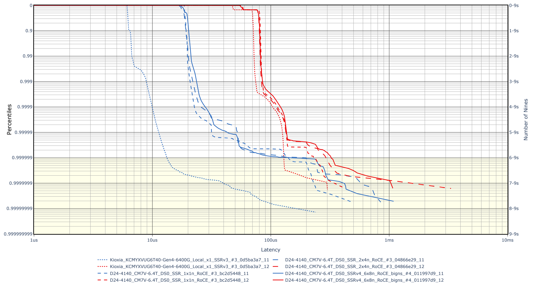
Latency Exceedance for Kioxia CM7-V
